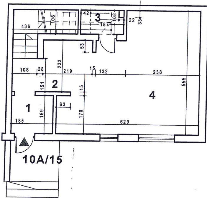
PARTER
