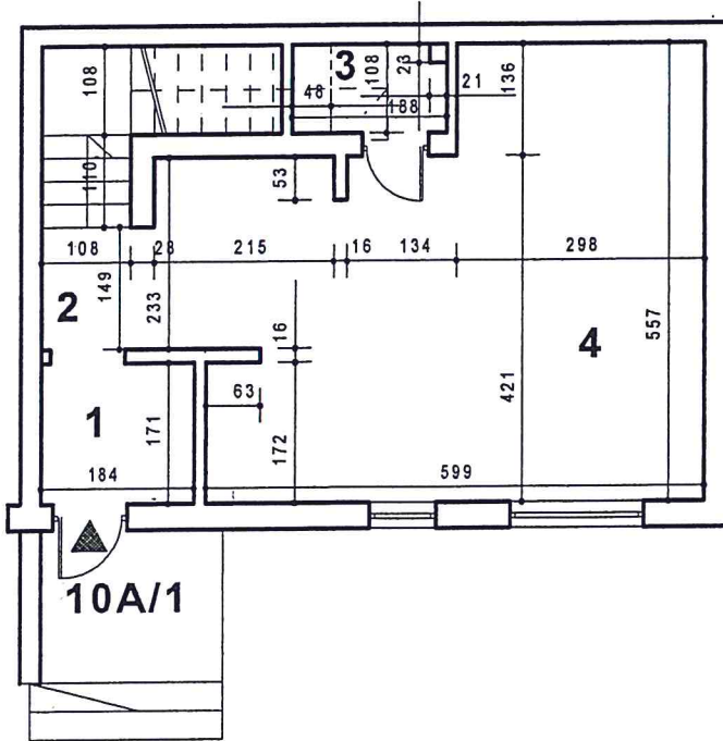
PARTER
