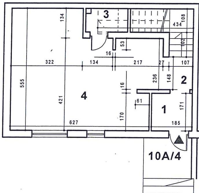
PARTER
